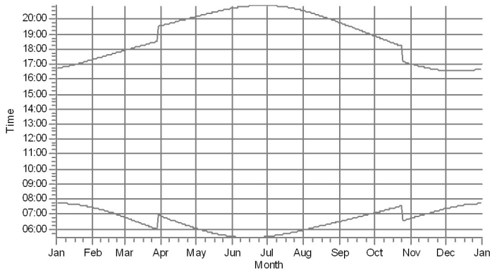
11: VESTAS V170-6.4 6400 170.0 !O! hub: 155.0 m (TOT: 240.0 m) (23)
